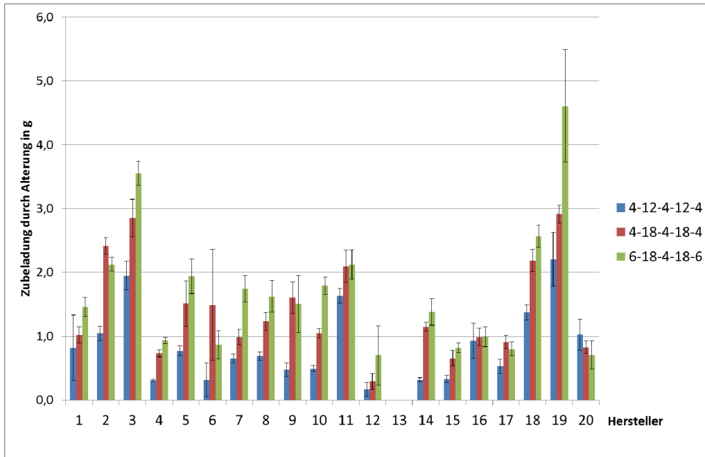
Figure 2 Average moisture uptake during ageing with 95 % confidence intervals
