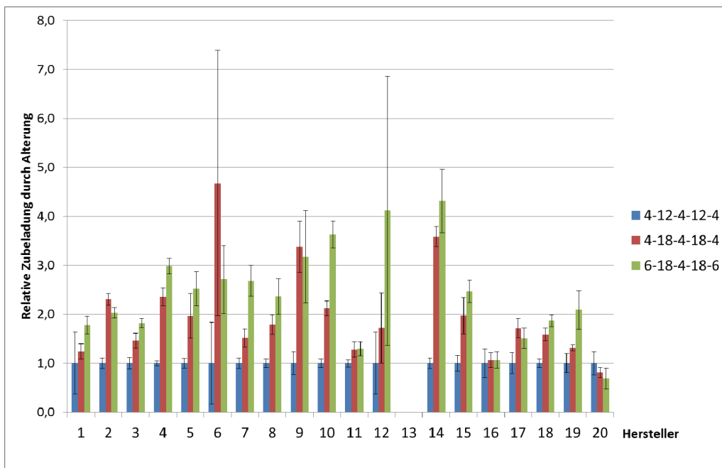
Figure 3 Average relative moisture uptake during ageing, normalized for each manufacturer individually with respect to its construction 1; with 95 % confidence intervals
