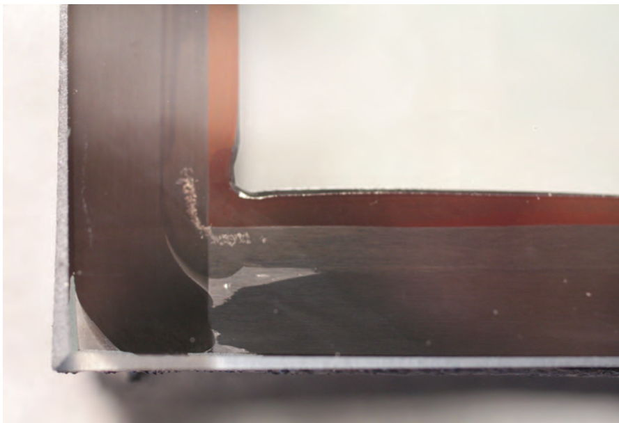
Figure 5 Insufficient butyl covering at the corner where the spacer has been widened by bending; air pockets (grey) in secondary sealant at the start/end point of the automatic sealing process
