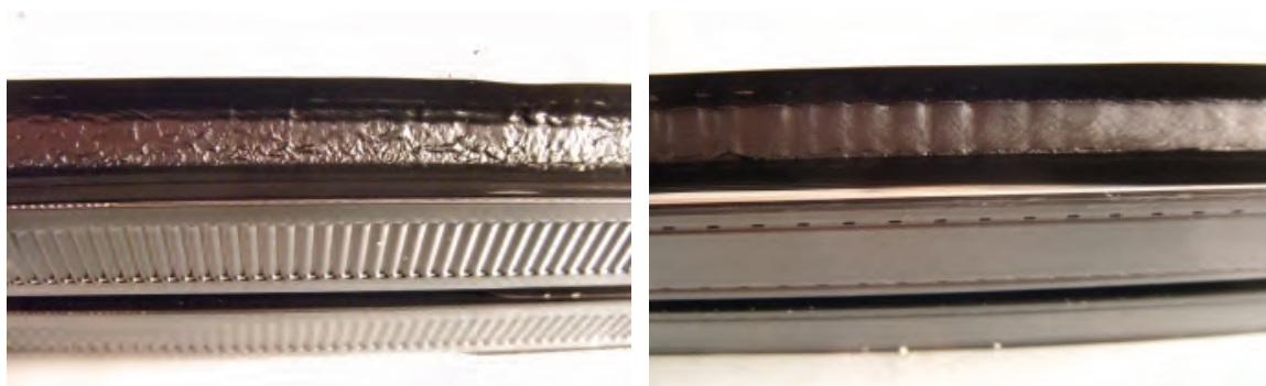
Figure 8 Cohesive failure in the butyl – no stringing
