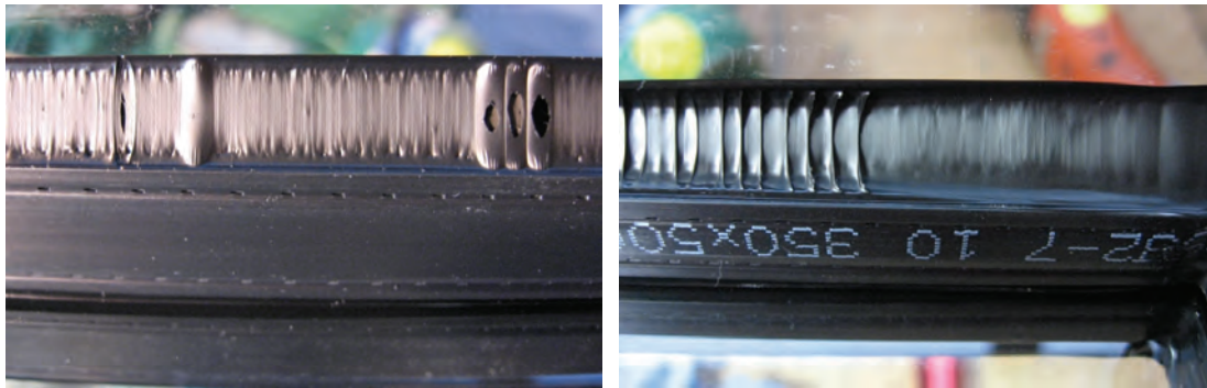
Figure 6 Example of butyl stringing in butterfly test: good adhesion – formation of a closed curtain of strings
