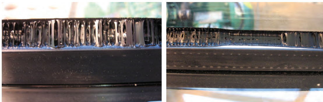
Figure 7 Example of stringing in butterfly test: patches with bad adhesion between butyl and spacer are visible
