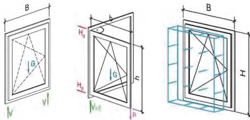
Figure 4 Loads on the window from the left to the right: Dead load, loads caused by opened sash, loads caused by wind
