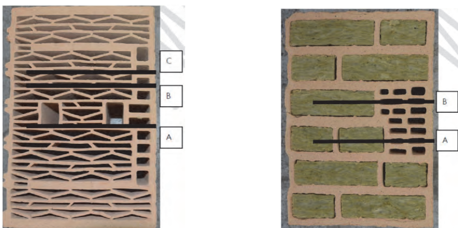
Figure 6 Reveal brick with pattern of cavities optimised with respect to the mechanical properties. Left: Filigree brick (brick type no. 50), Right: Large chamber brick (brick type no. 60)
