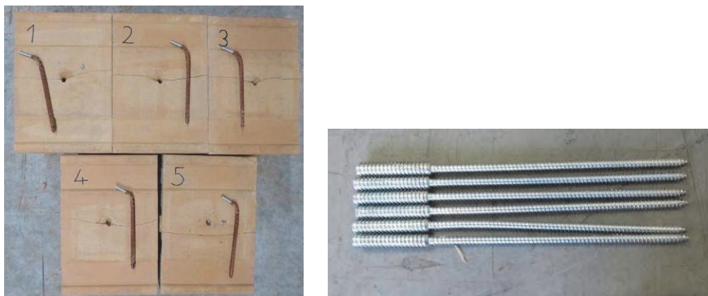
Figure 11 Appearance of the fixing material at the end of the respective test Left: Small test of parts Right: Components test
