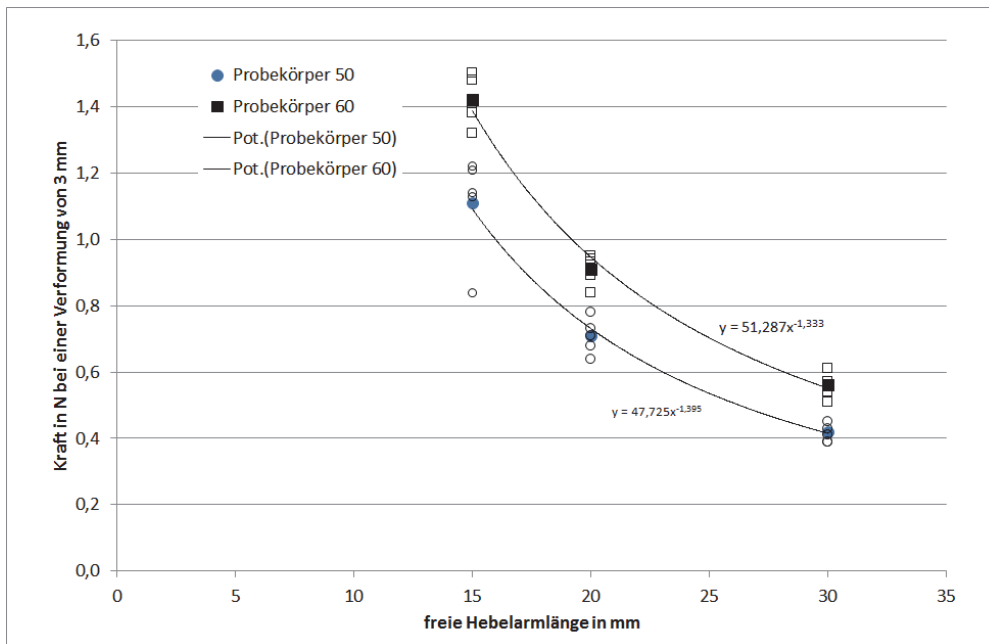
Figure 5 Graphical illustration of the correlation between the free lever arm length and load for a deformation of 3°mm. Apart from the mean values of the measurement (filled marker), even the individual values are entered (data points not filled up). In addition, compensation curves have been marked assuming a potential correlation.
