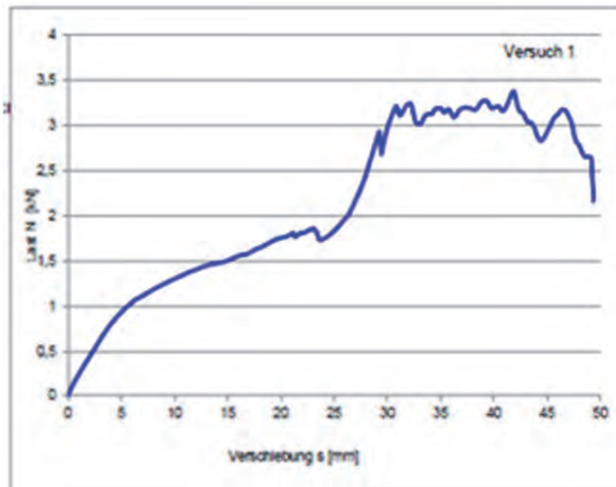
Figure 10 Typical force-displacement diagram in the course of the small test for parts
