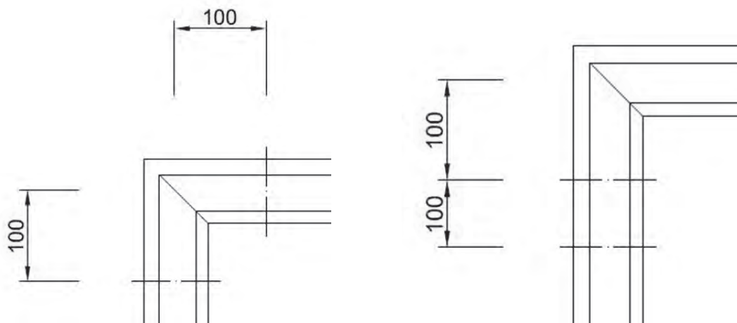
Figure 8 Group fastening for better load transfer with "point loads" Left: Symmetric group fastening using an example of a stay bearing Right: Double fastening using an example of a stay bearing
