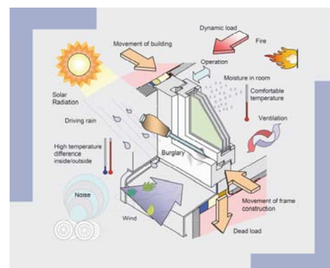
Fig. 1 A window is exposed to many influences – the correct installation increases service life and functionality
